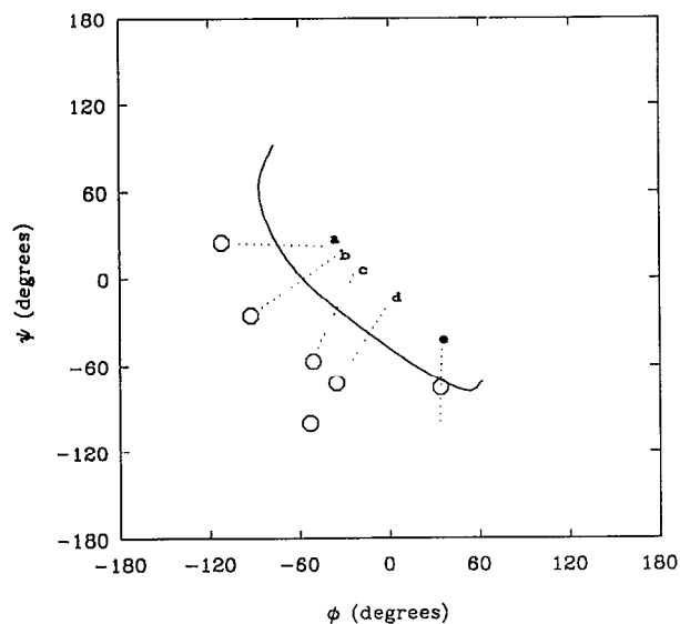
FIG. 5. Reaction path in water for the alanine dipeptide. The peaks of the probability distributions along the orthogonal coordinate are denoted by circles. The two circles in one of the orthogonal runs correspond to the two peaks of the probability distribution. For comparison, the vacuum path is shown by the solid line.
