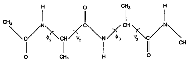
FIG. 6. The blocked alanine tripeptide used as a model for a reverse turn. The alanine dipeptide has one alanyl residue [NHCH(CH 3 )CO] less.
